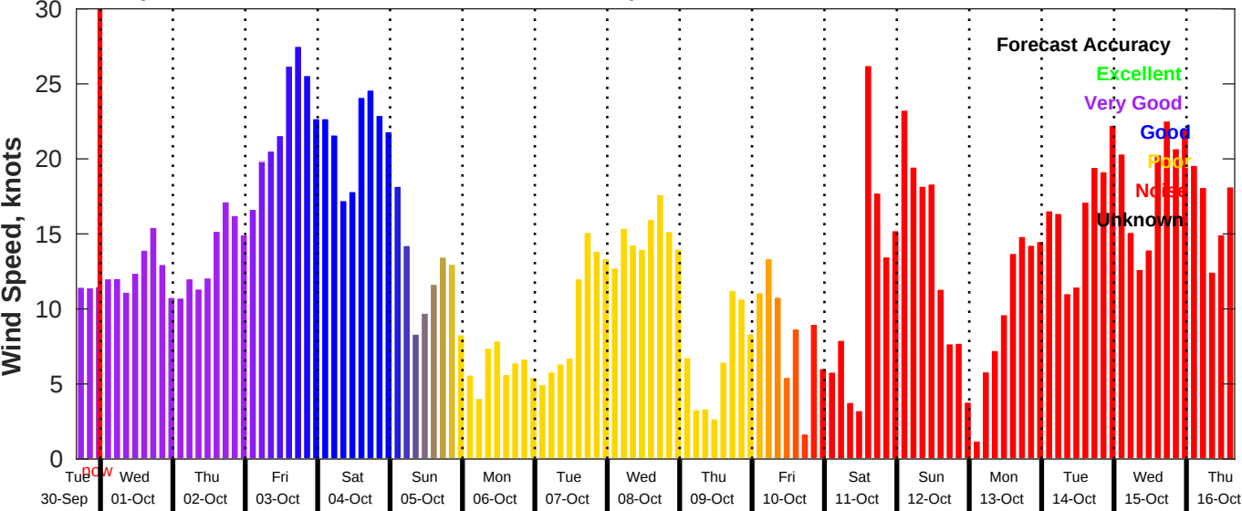
GFS Wind Speed Forecast for NDBC 46054 from 30-Sep-2025 16:00:00 to 16-Oct-2025 16:00:00
