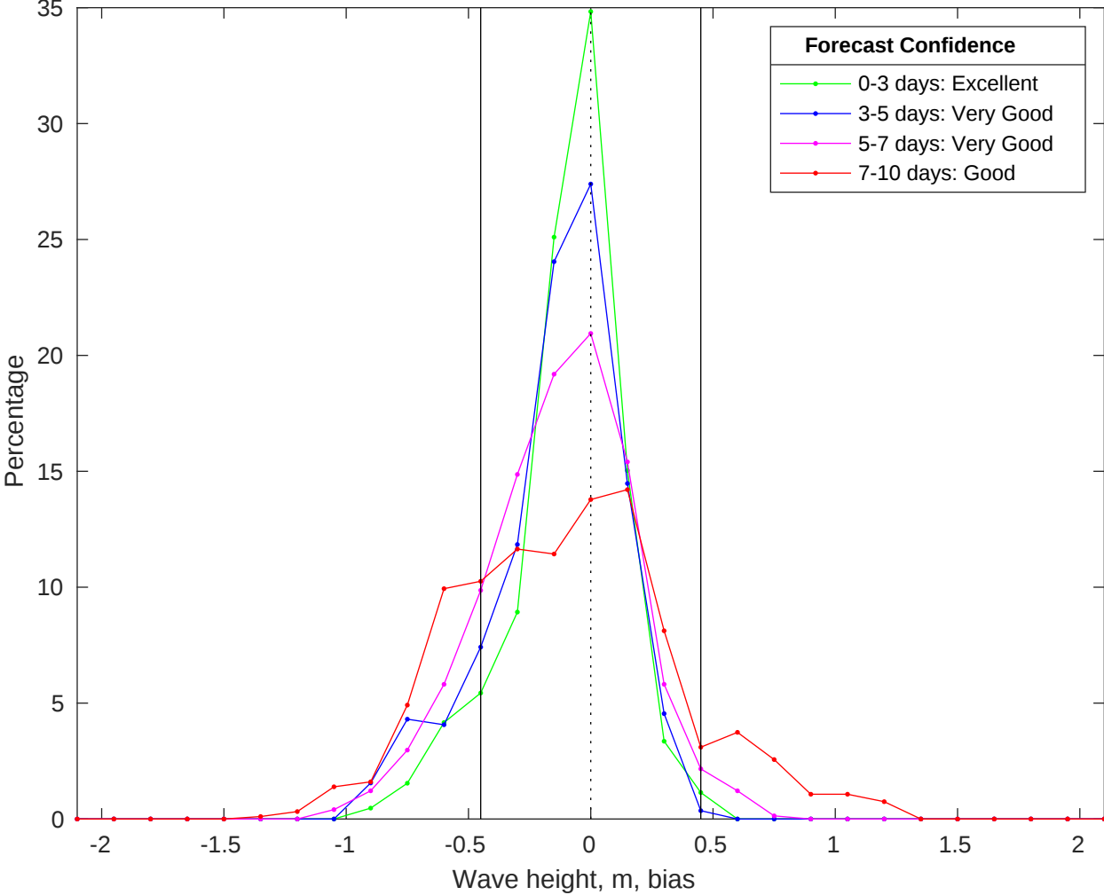
NDBC 46069 vs CMEMS Waves Bias Histogram: 01-Oct-2025
