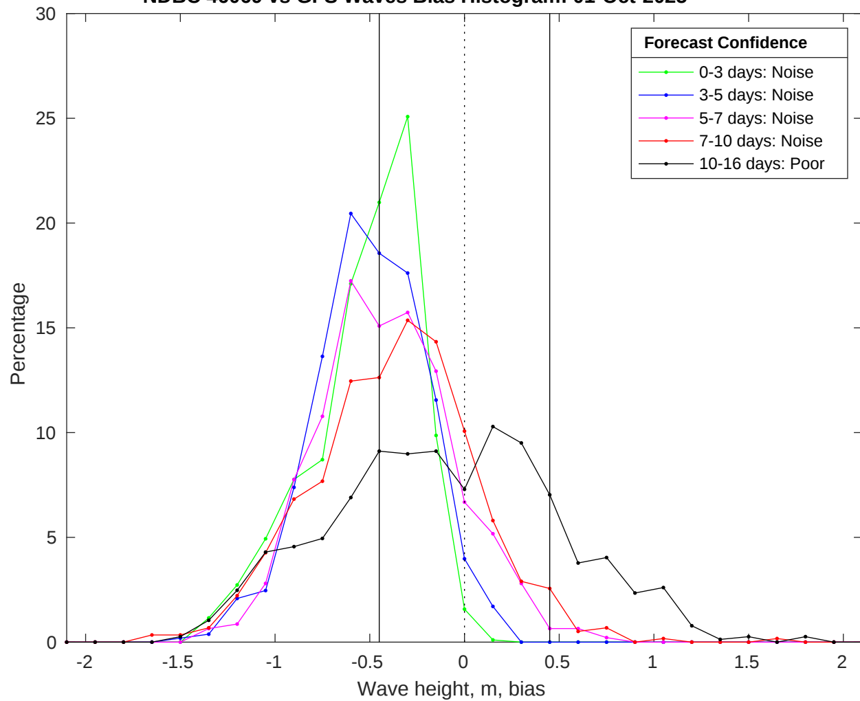
NDBC 46069 vs GFS Waves Bias Histogram: 01-Oct-2025
