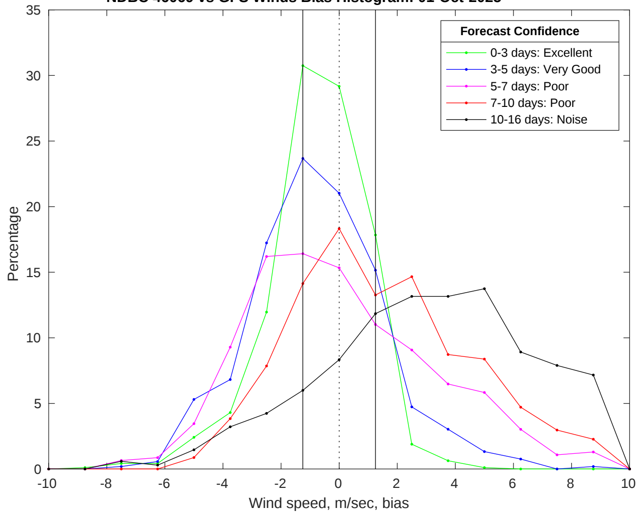
NDBC 46069 vs GFS Winds Bias Histogram: 01-Oct-2025
