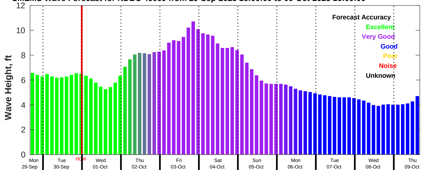
CMEMS Wave Forecast for NDBC 46069 from 29-Sep-2025 16:00:00 to 09-Oct-2025 16:00:00
