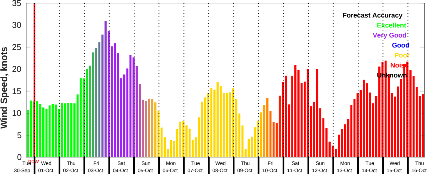
GFS Wind Speed Forecast for NDBC 46069 from 30-Sep-2025 16:00:00 to 16-Oct-2025 16:00:00
