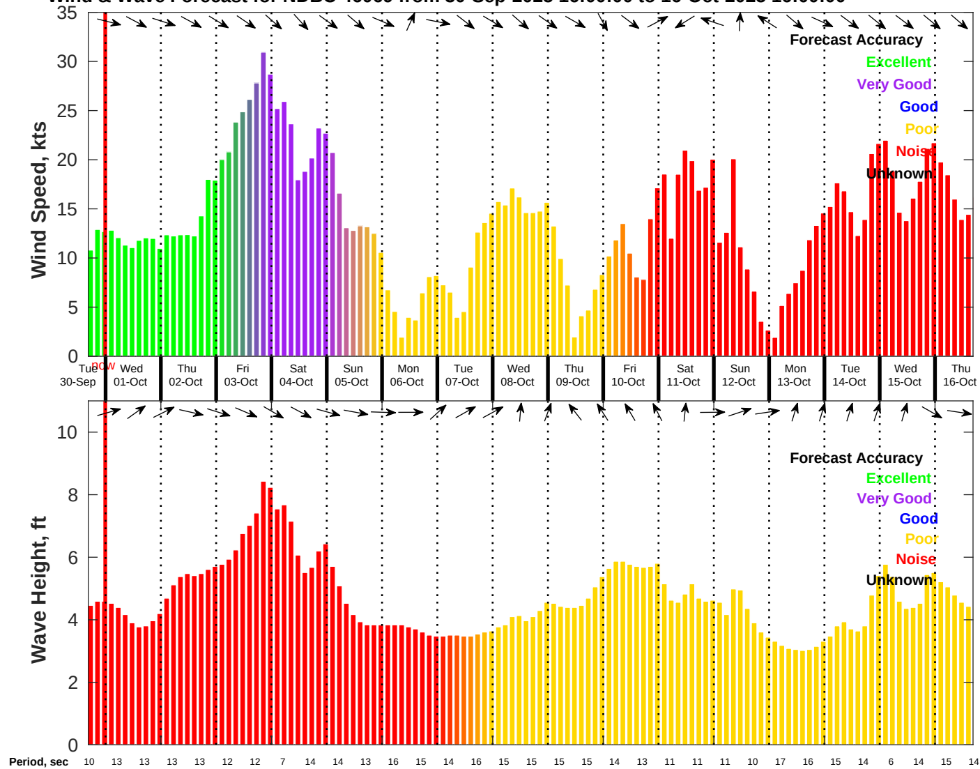
Wind & Wave Forecast for NDBC 46069 from 30-Sep-2025 16:00:00 to 16-Oct-2025 16:00:00
