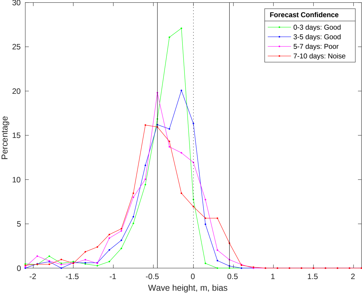
NDBC 51209 vs CMEMS Waves Bias Histogram: 01-Oct-2025
