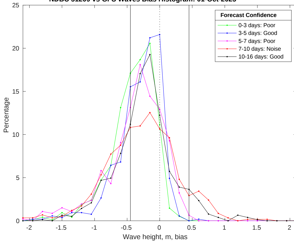
NDBC 51209 vs GFS Waves Bias Histogram: 01-Oct-2025
