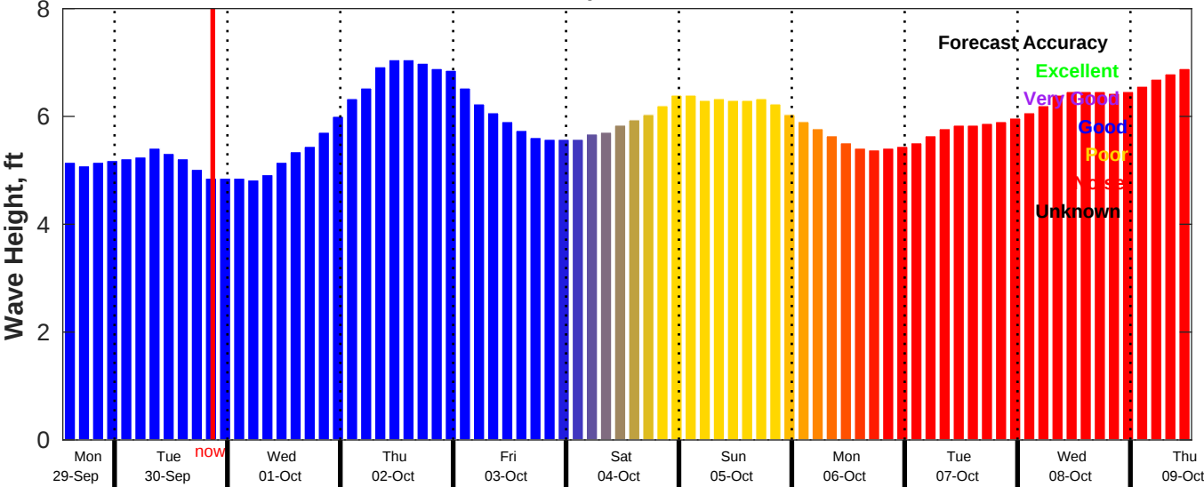
CMEMS Wave Forecast for NDBC 51209 from 29-Sep-2025 13:00:00 to 09-Oct-2025 13:00:00
