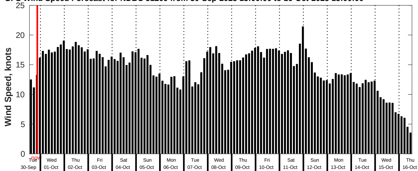
GFS Wind Speed Forecast for NDBC 51209 from 30-Sep-2025 13:00:00 to 16-Oct-2025 13:00:00
