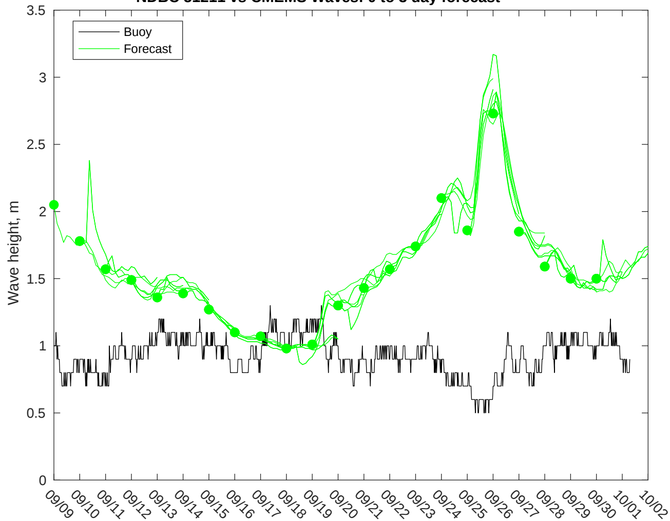
NDBC 51211 vs CMEMS Waves: 0 to 3 day forecast
