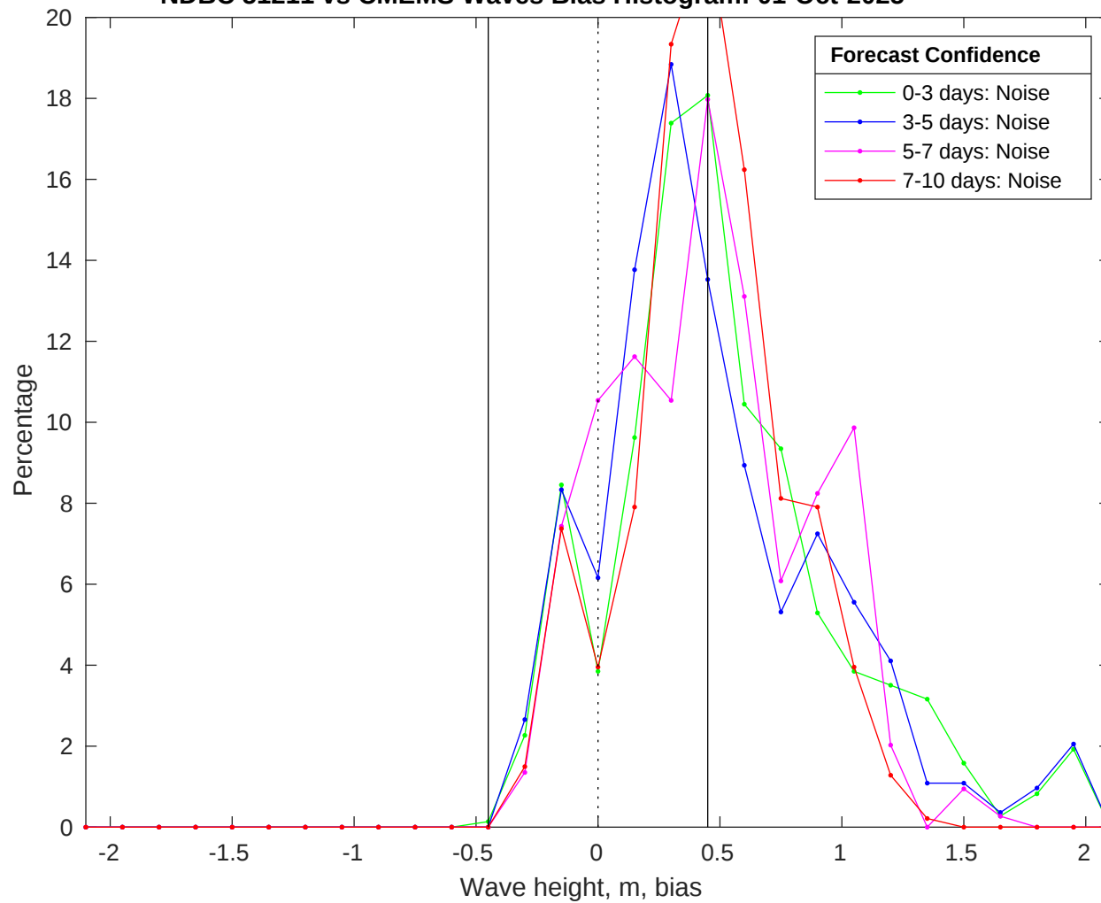
NDBC 51211 vs CMEMS Waves Bias Histogram: 01-Oct-2025
