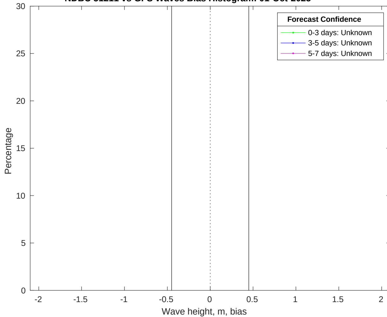
NDBC 51211 vs GFS Waves Bias Histogram: 01-Oct-2025
