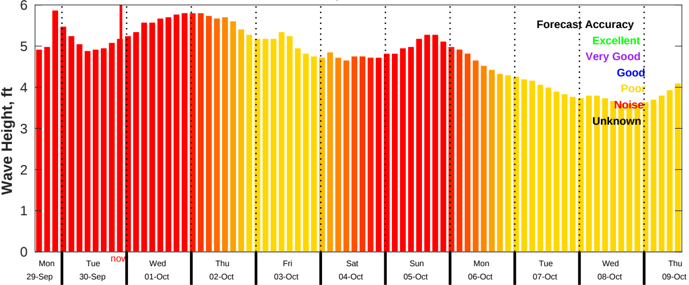
CMEMS Wave Forecast for NDBC 51211 from 29-Sep-2025 14:00:00 to 09-Oct-2025 14:00:00
