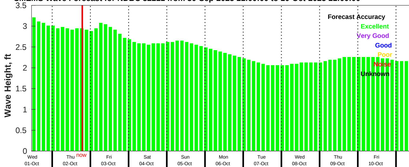
CMEMS Wave Forecast for NDBC 52211 from 30-Sep-2025 11:00:00 to 10-Oct-2025 11:00:00
