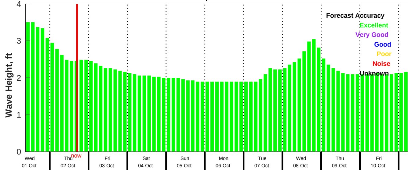
CMEMS Wave Forecast for NDBC 52212 from 30-Sep-2025 09:00:00 to 10-Oct-2025 09:00:00
