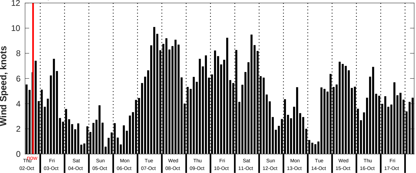
GFS Wind Speed Forecast for NDBC 52212 from 01-Oct-2025 09:00:00 to 17-Oct-2025 09:00:00
