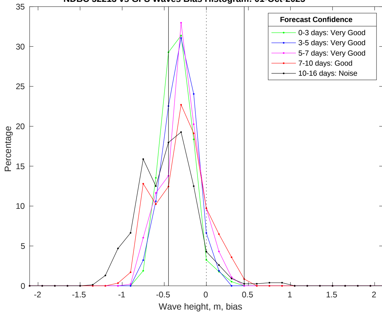
NDBC 52213 vs GFS Waves Bias Histogram: 01-Oct-2025
