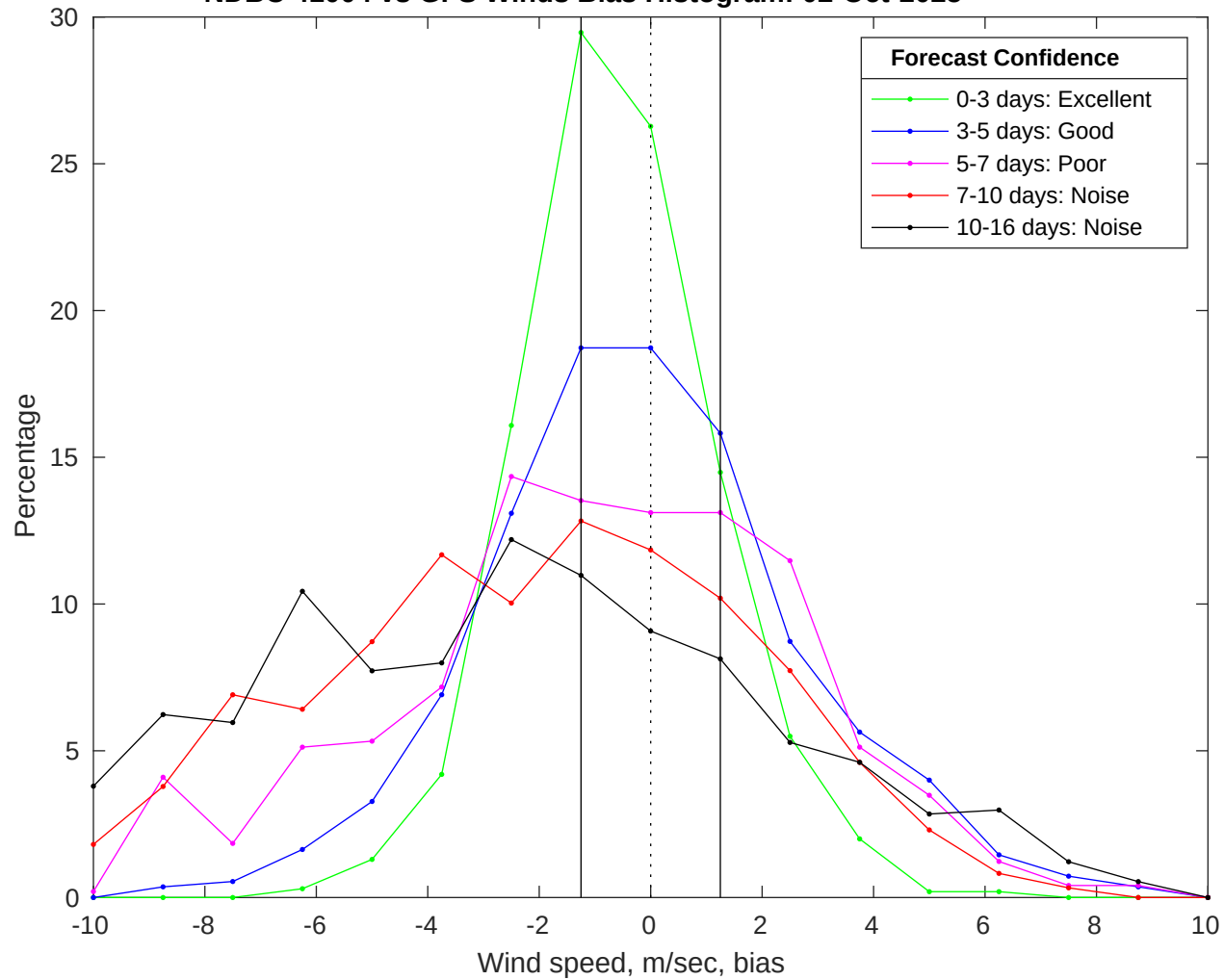
NDBC 41004 vs GFS Winds Bias Histogram: 02-Oct-2025
