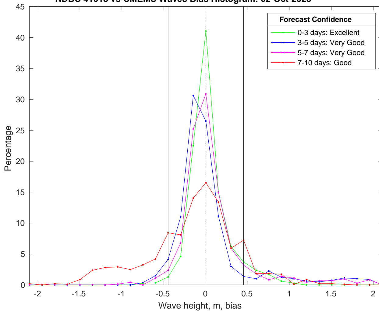
NDBC 41013 vs CMEMS Waves Bias Histogram: 02-Oct-2025
