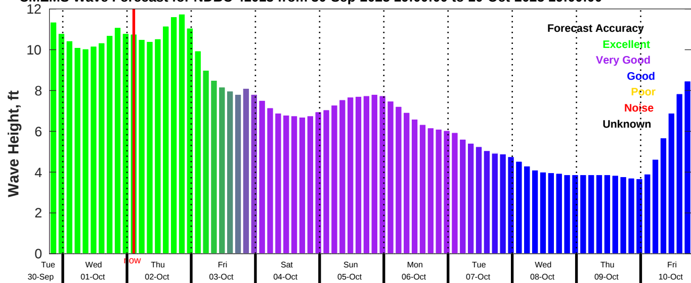
CMEMS Wave Forecast for NDBC 41013 from 30-Sep-2025 19:00:00 to 10-Oct-2025 19:00:00
