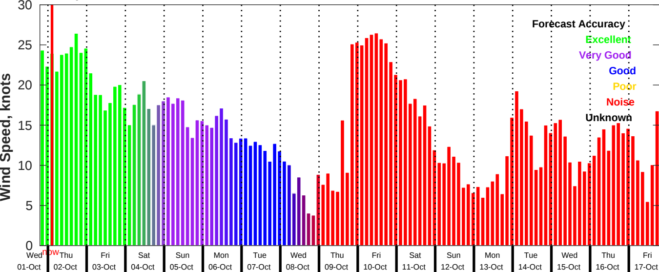
GFS Wind Speed Forecast for NDBC 41013 from 01-Oct-2025 19:00:00 to 17-Oct-2025 19:00:00
