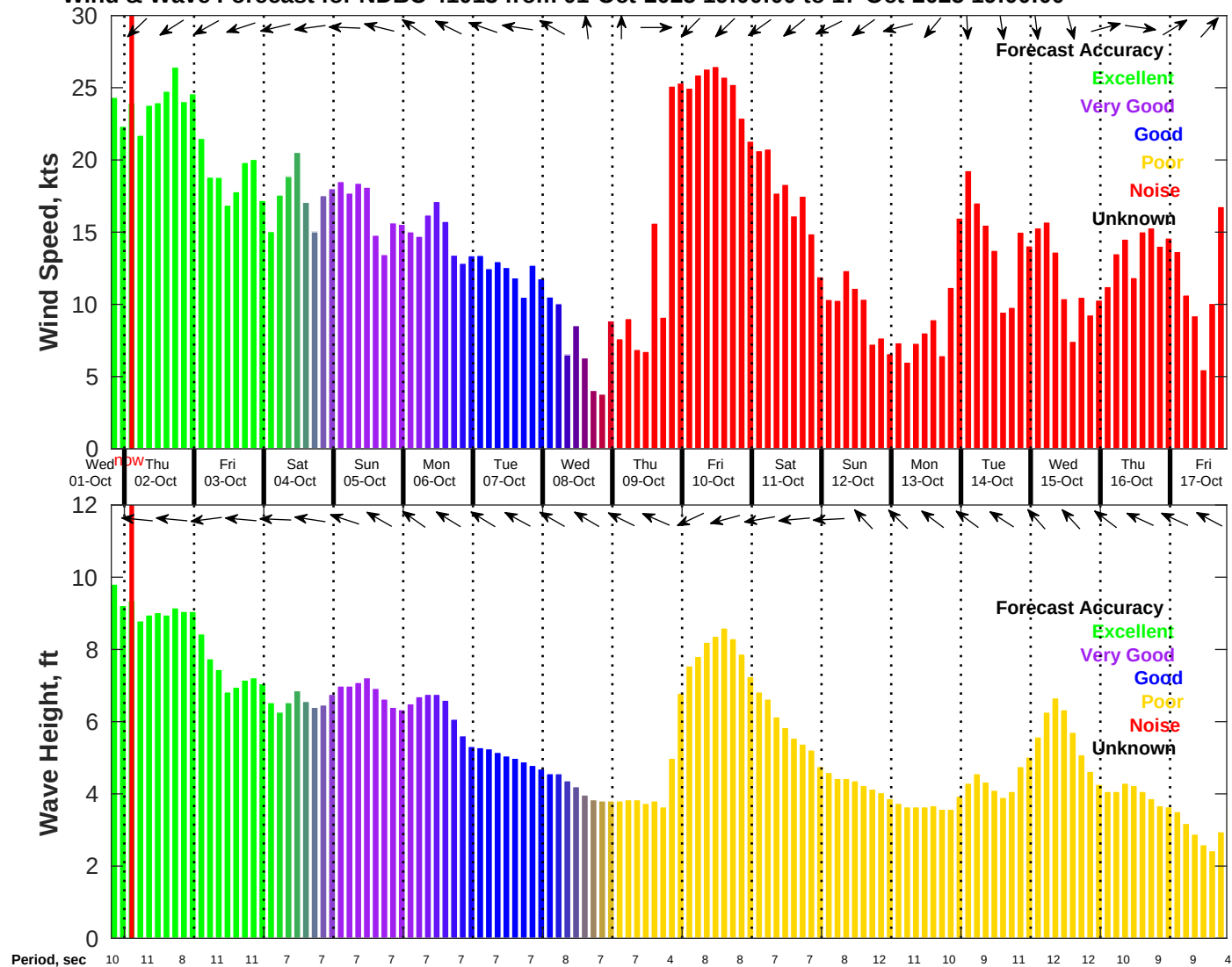
Wind & Wave Forecast for NDBC 41013 from 01-Oct-2025 19:00:00 to 17-Oct-2025 19:00:00
