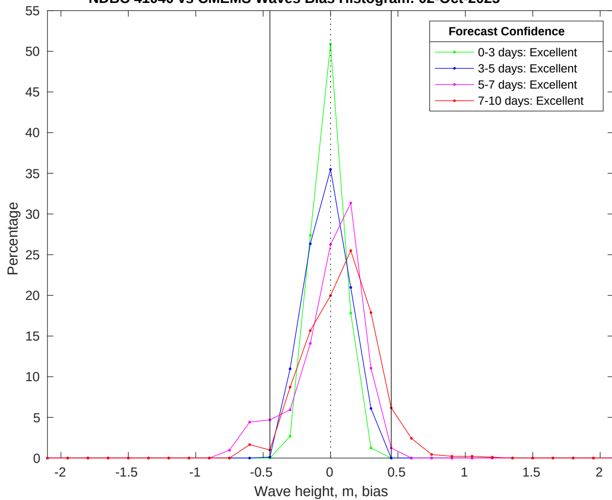
NDBC 41040 vs CMEMS Waves Bias Histogram: 02-Oct-2025
