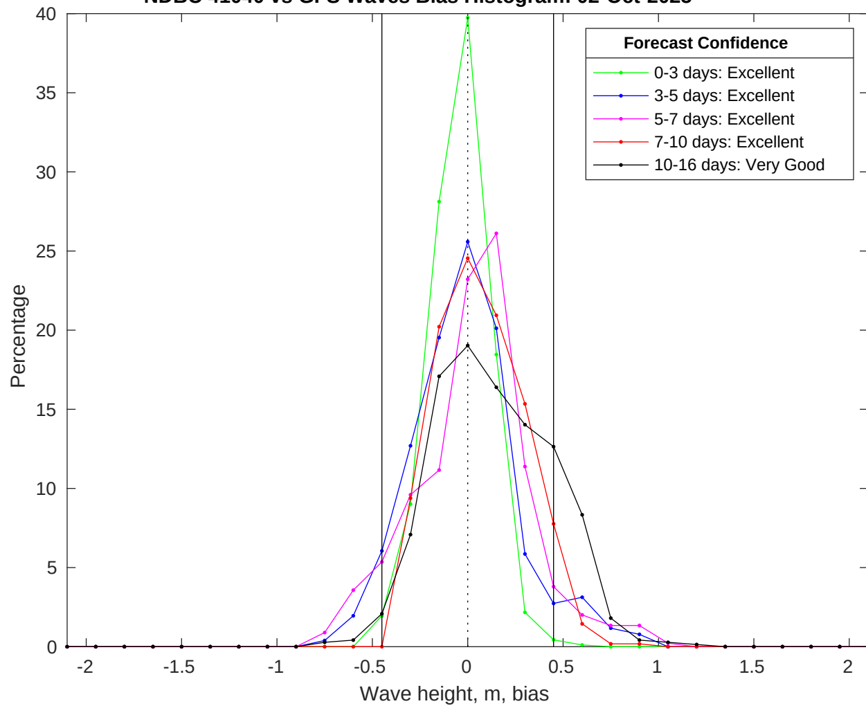
NDBC 41040 vs GFS Waves Bias Histogram: 02-Oct-2025
