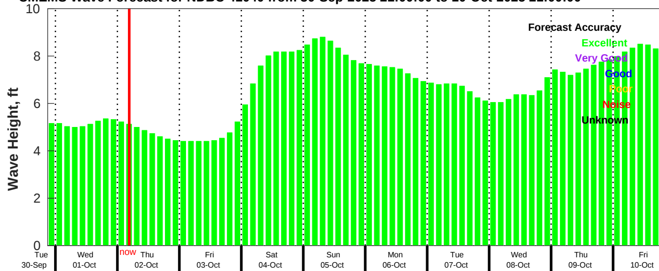
CMEMS Wave Forecast for NDBC 41040 from 30-Sep-2025 21:00:00 to 10-Oct-2025 21:00:00
