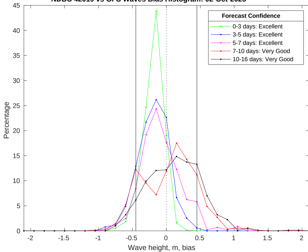
NDBC 42019 vs GFS Waves Bias Histogram: 02-Oct-2025
