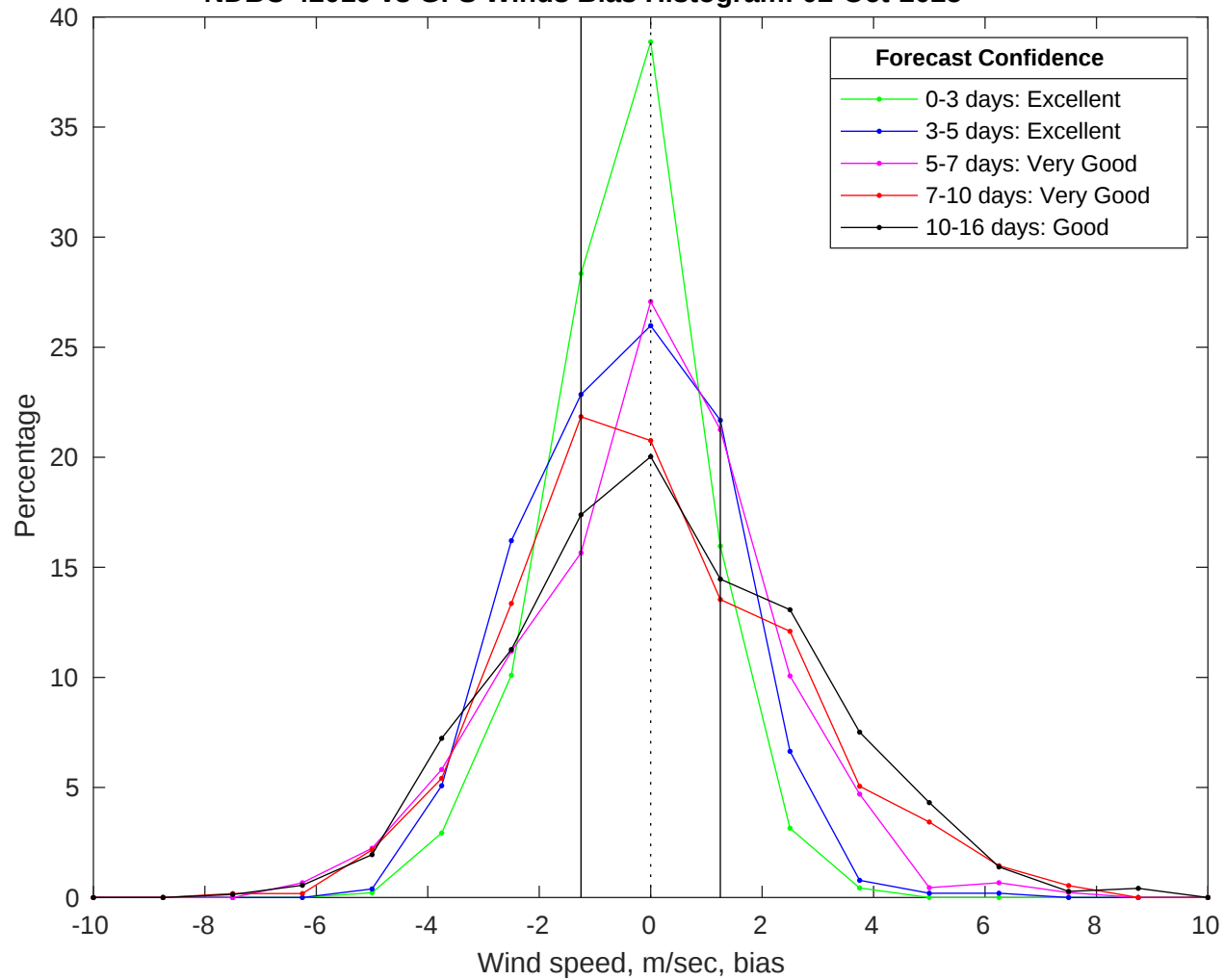
NDBC 42019 vs GFS Winds Bias Histogram: 02-Oct-2025
