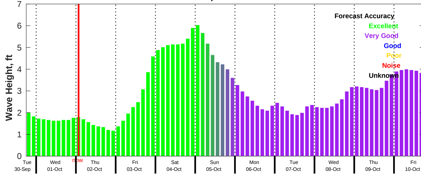
CMEMS Wave Forecast for NDBC 42019 from 30-Sep-2025 18:00:00 to 10-Oct-2025 18:00:00
