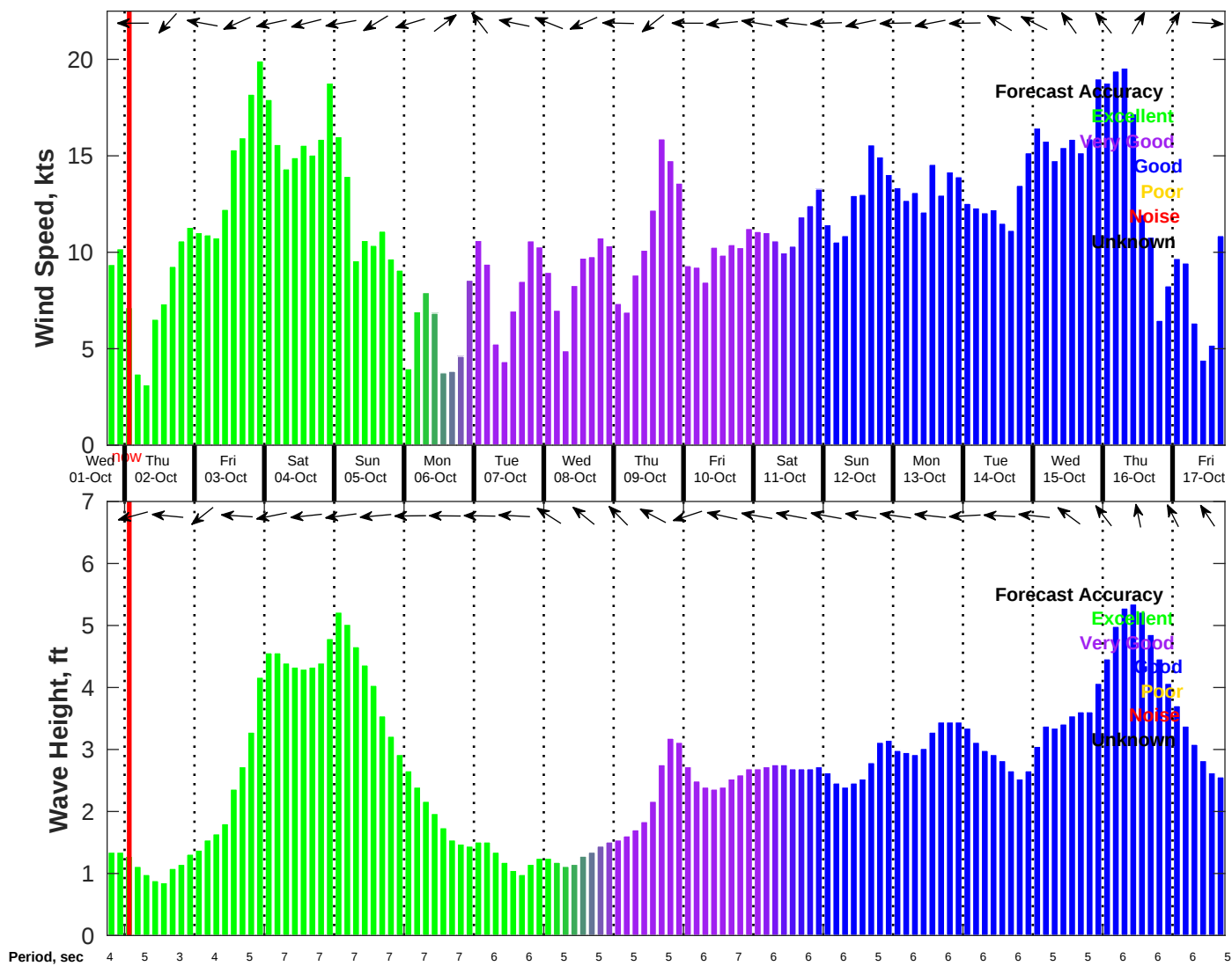
Wind & Wave Forecast for NDBC 42019 from 01-Oct-2025 18:00:00 to 17-Oct-2025 18:00:00
