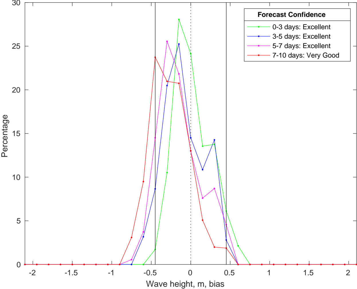
NDBC 42020 vs CMEMS Waves Bias Histogram: 02-Oct-2025
