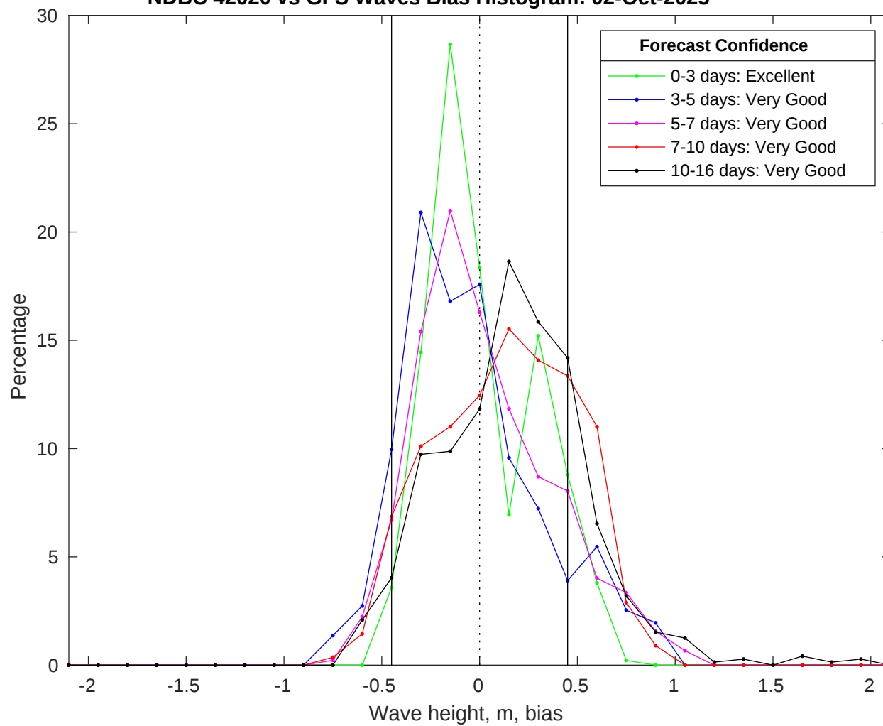
NDBC 42020 vs GFS Waves Bias Histogram: 02-Oct-2025
