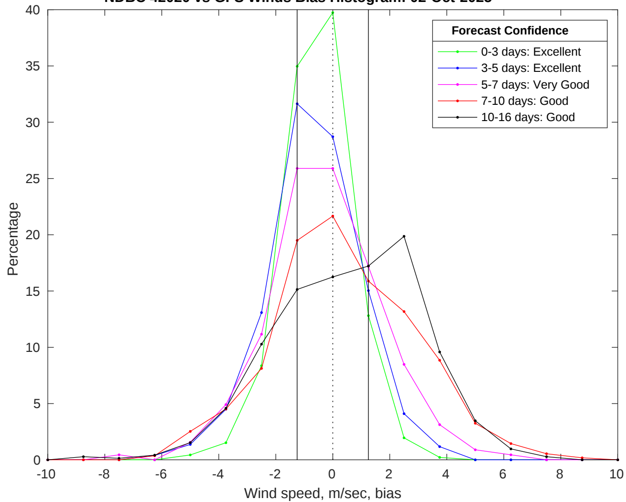
NDBC 42020 vs GFS Winds Bias Histogram: 02-Oct-2025
