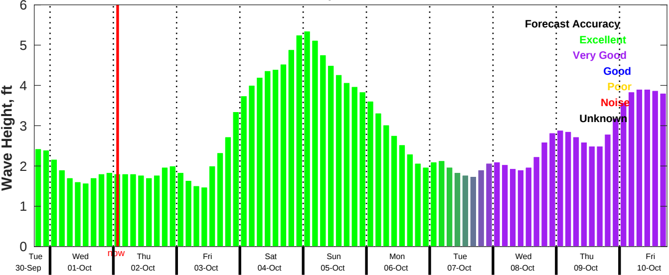
CMEMS Wave Forecast for NDBC 42020 from 30-Sep-2025 18:00:00 to 10-Oct-2025 18:00:00
