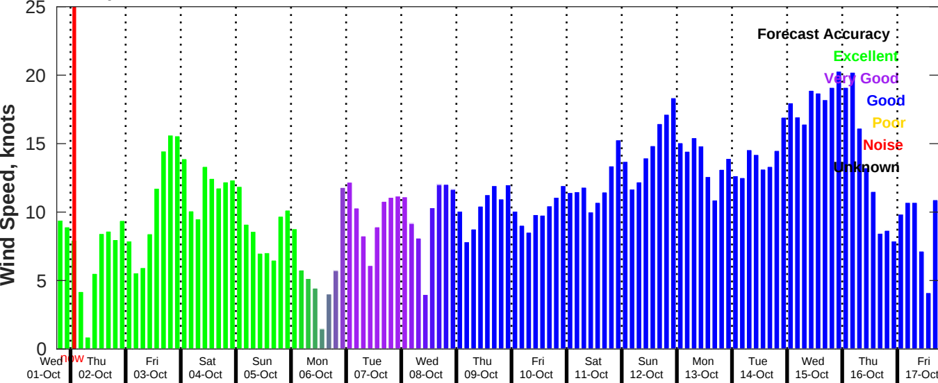
GFS Wind Speed Forecast for NDBC 42020 from 01-Oct-2025 18:00:00 to 17-Oct-2025 18:00:00
