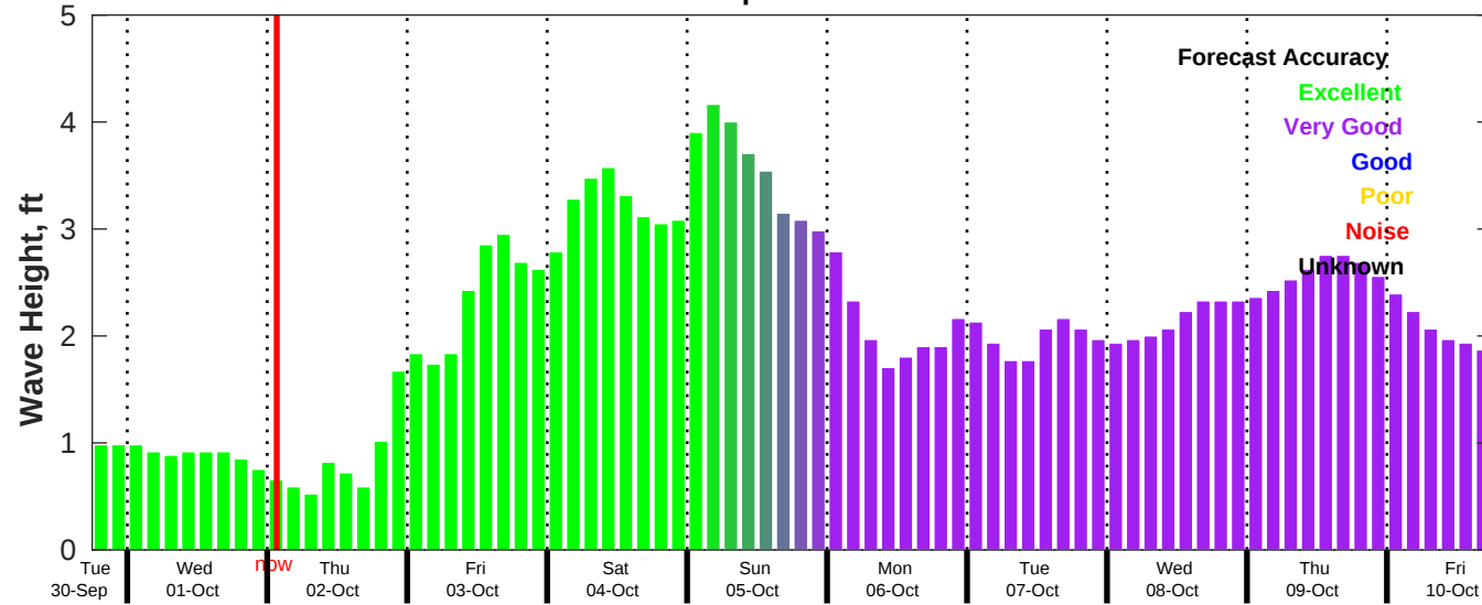
CMEMS Wave Forecast for NDBC 42035 from 30-Sep-2025 18:00:00 to 10-Oct-2025 18:00:00
