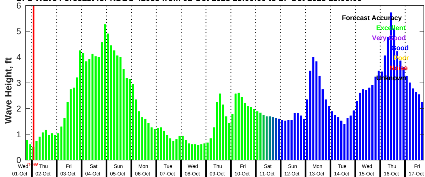
GFS Wave Forecast for NDBC 42035 from 01-Oct-2025 18:00:00 to 17-Oct-2025 18:00:00
