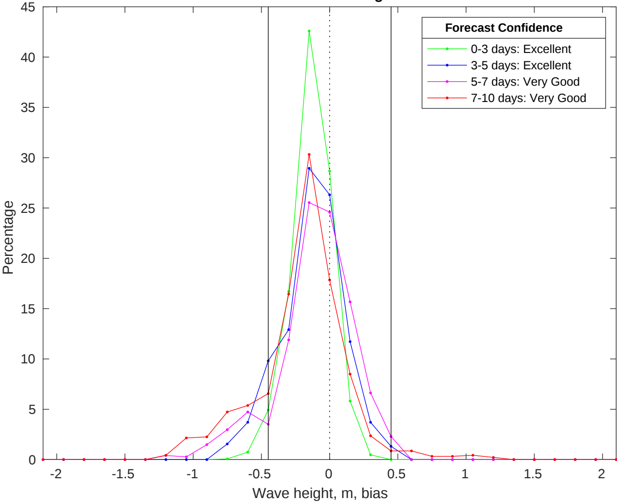
NDBC 42036 vs CMEMS Waves Bias Histogram: 02-Oct-2025
