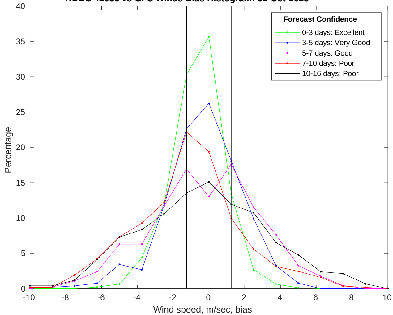
NDBC 42036 vs GFS Winds Bias Histogram: 02-Oct-2025
