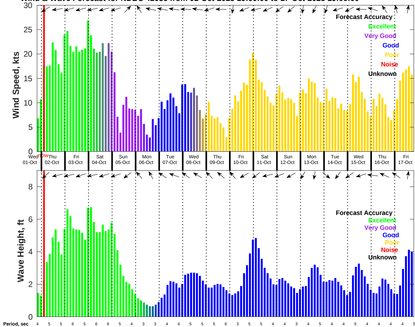
Wind & Wave Forecast for NDBC 42036 from 01-Oct-2025 19:00:00 to 17-Oct-2025 19:00:00
