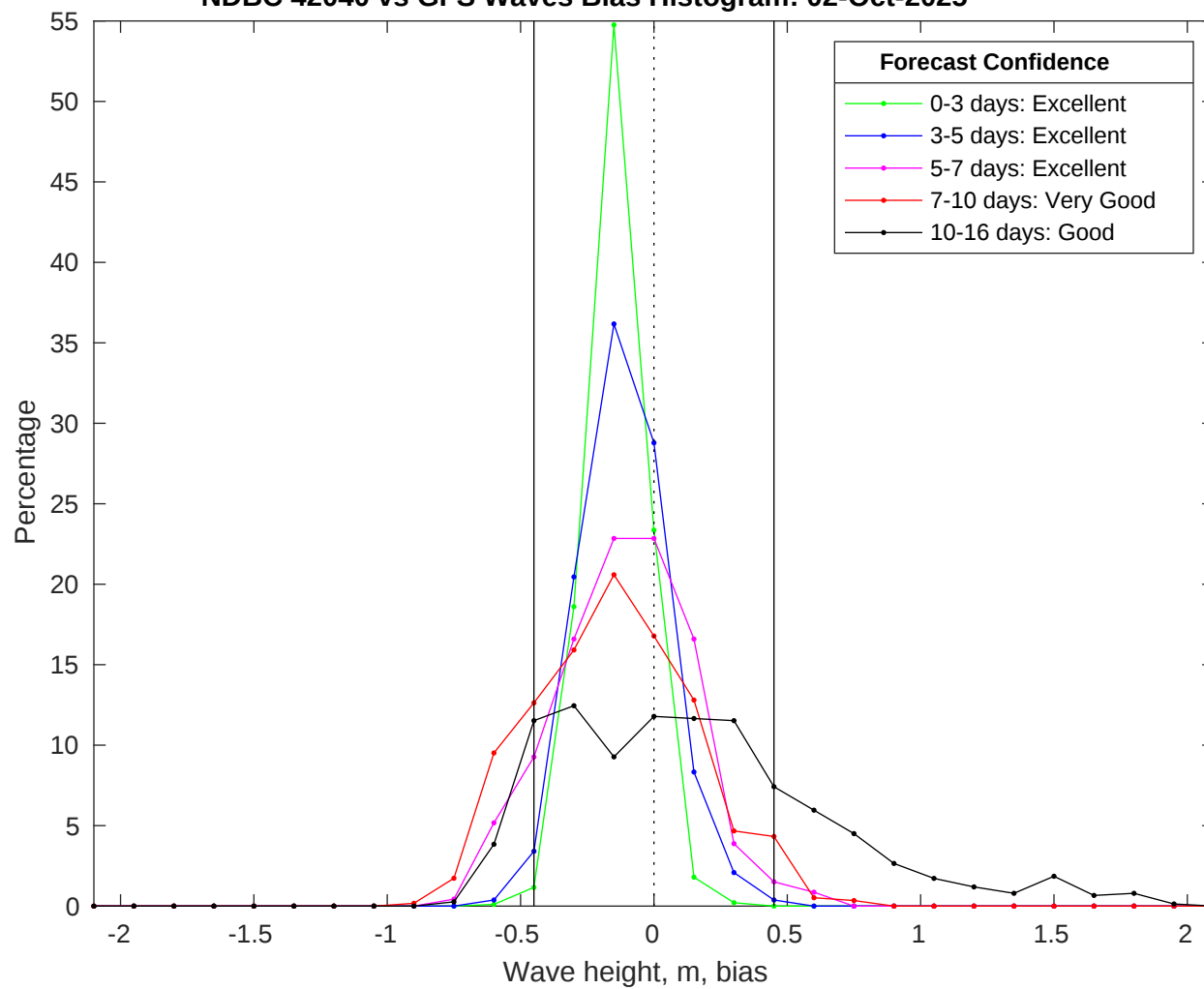
NDBC 42040 vs GFS Waves Bias Histogram: 02-Oct-2025
