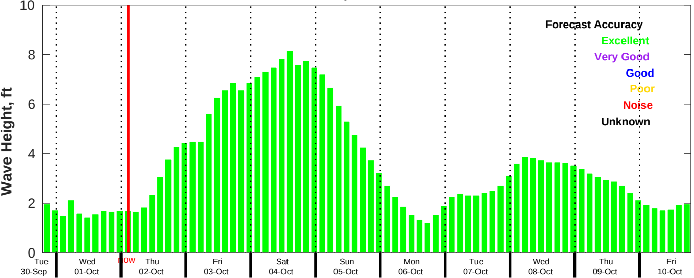
CMEMS Wave Forecast for NDBC 42040 from 30-Sep-2025 19:00:00 to 10-Oct-2025 19:00:00
