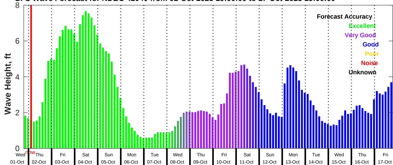
GFS Wave Forecast for NDBC 42040 from 01-Oct-2025 19:00:00 to 17-Oct-2025 19:00:00
