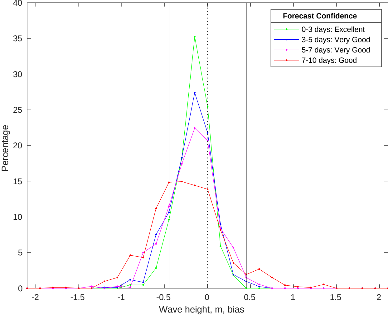
NDBC 46011 vs CMEMS Waves Bias Histogram: 02-Oct-2025
