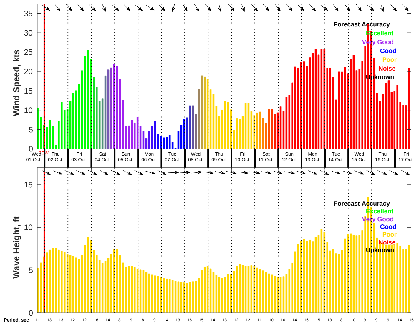
Wind & Wave Forecast for NDBC 46011 from 01-Oct-2025 16:00:00 to 17-Oct-2025 16:00:00
