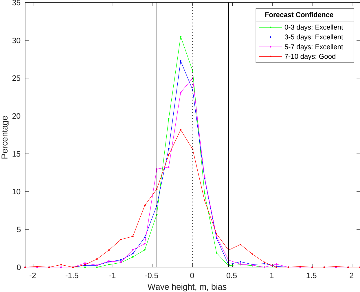
NDBC 46028 vs CMEMS Waves Bias Histogram: 02-Oct-2025
