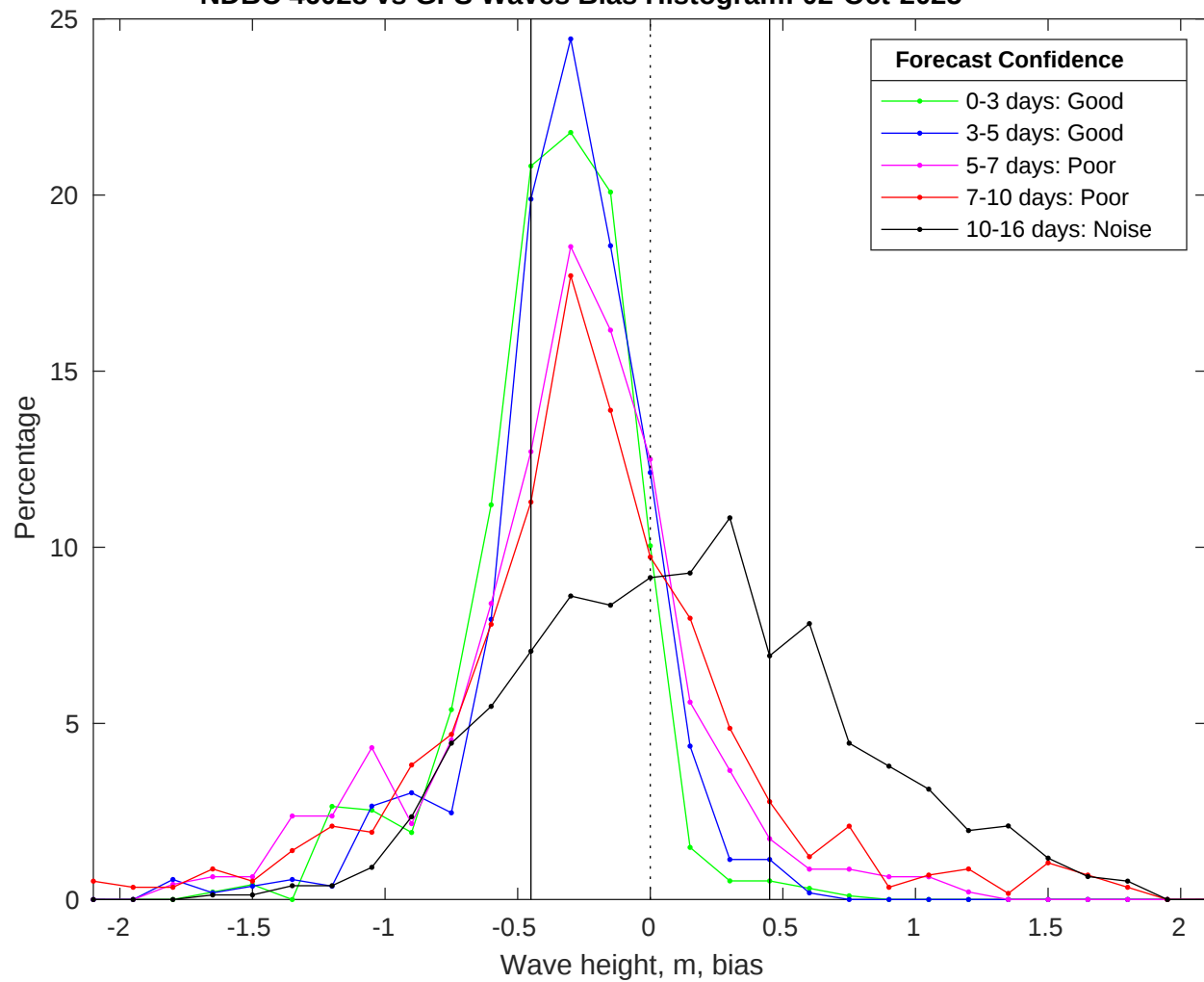
NDBC 46028 vs GFS Waves Bias Histogram: 02-Oct-2025
