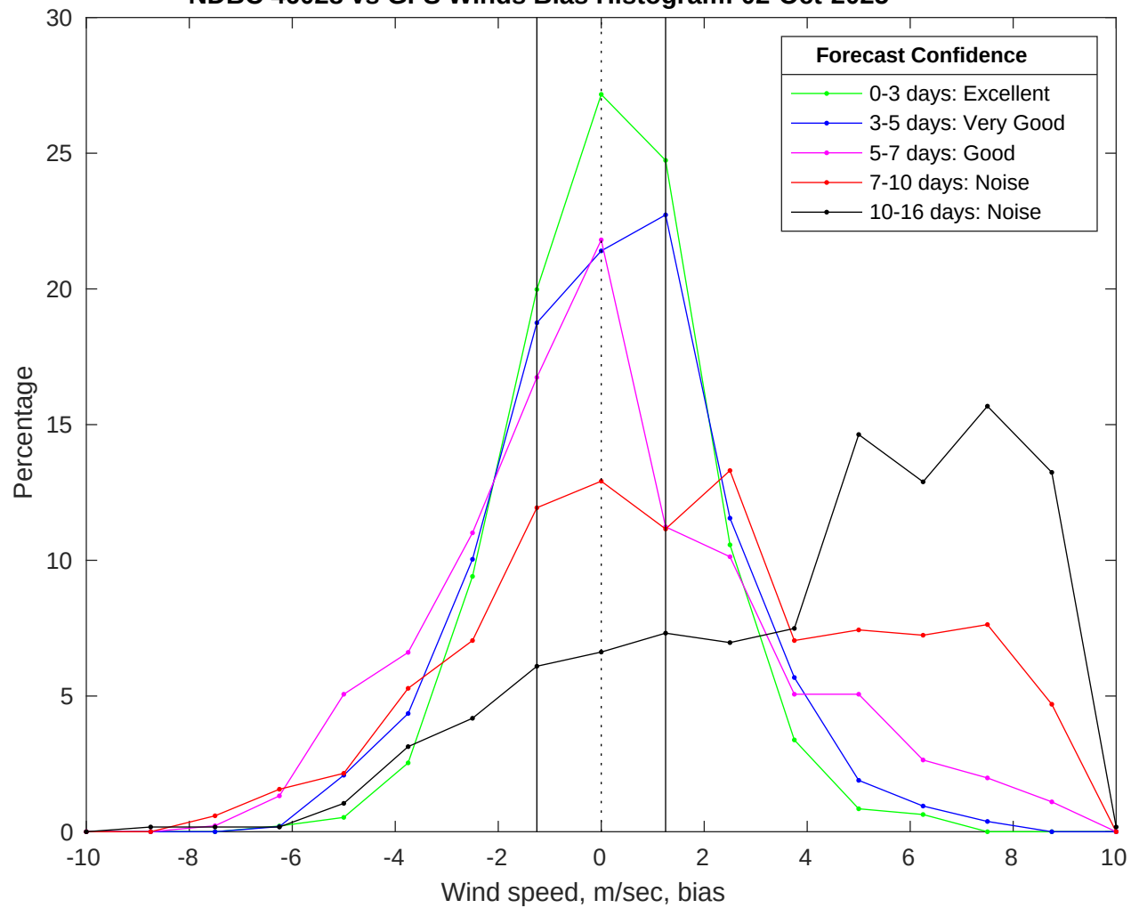
NDBC 46028 vs GFS Winds Bias Histogram: 02-Oct-2025
