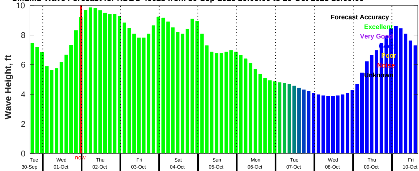
CMEMS Wave Forecast for NDBC 46028 from 30-Sep-2025 16:00:00 to 10-Oct-2025 16:00:00
